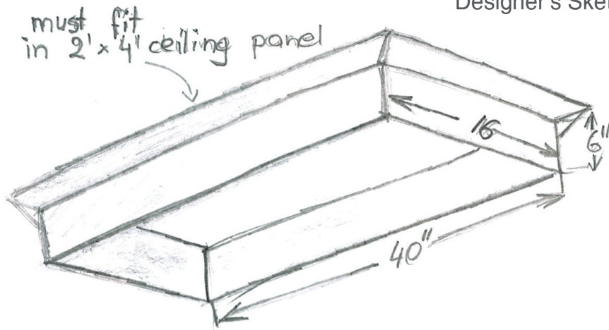
Designer's Sketch
